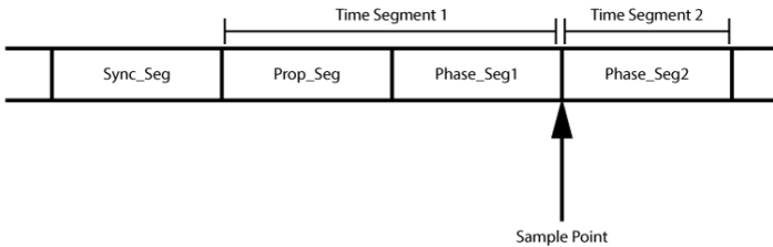
Figure 9: Bit Timing
