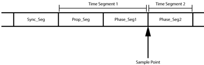
Figure 8: Bit Timing
