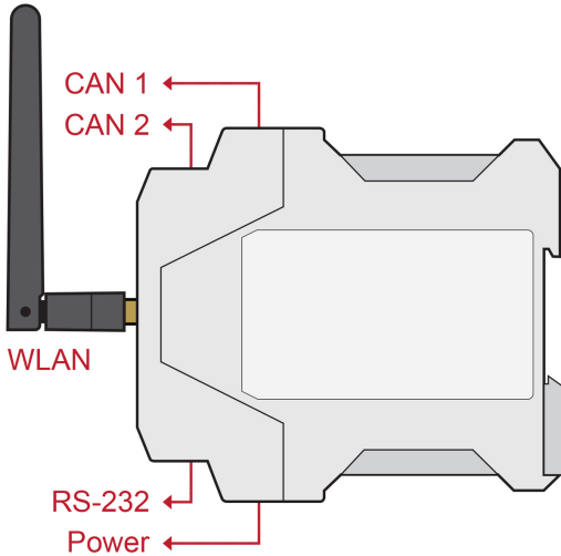
Figure 1: Position of the connectors
